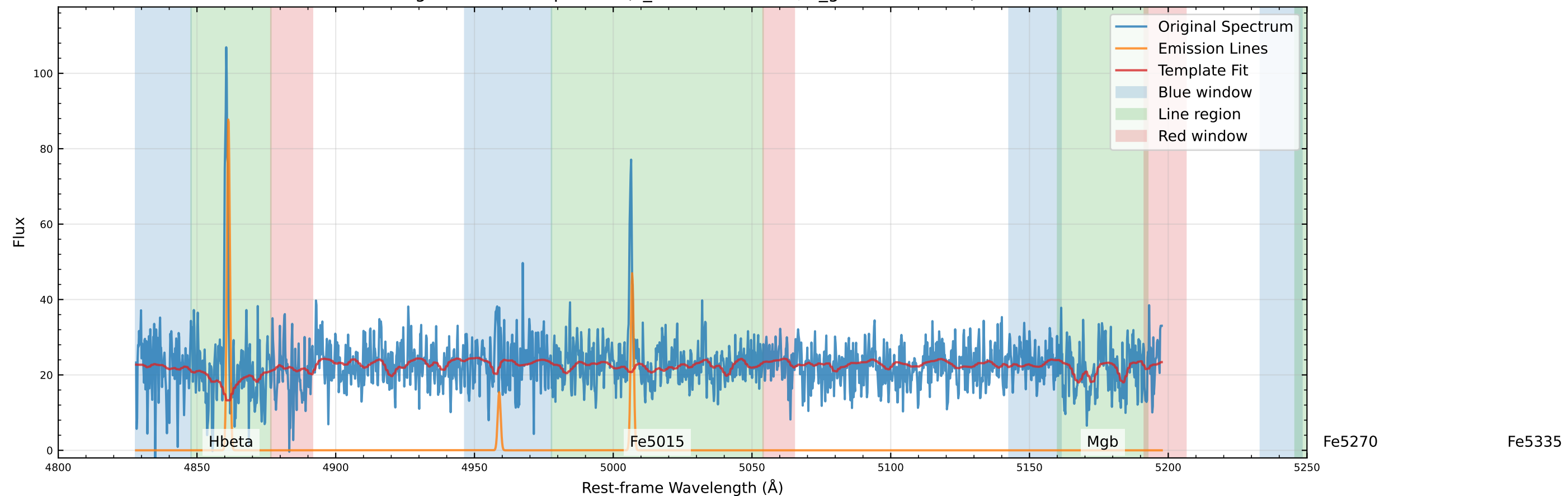
Original Data Comparison (v_star=-62.2 km/s, v_gas=-45.0 km/s)
