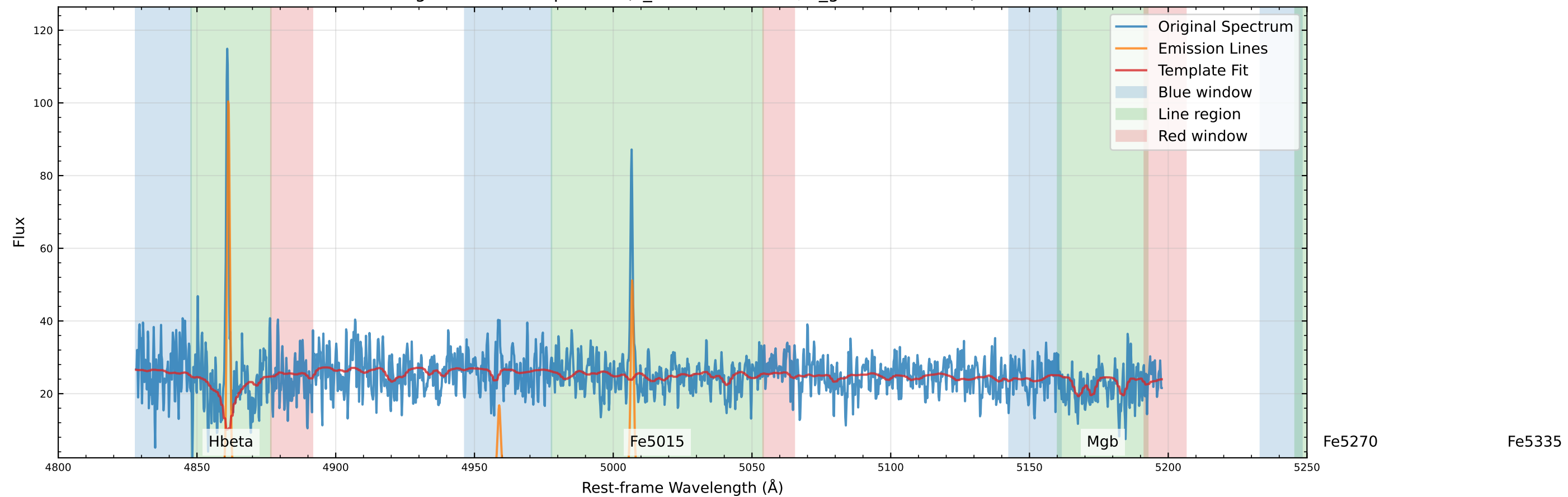
Original Data Comparison (v_star=-36.2 km/s, v_gas=-21.9 km/s)
