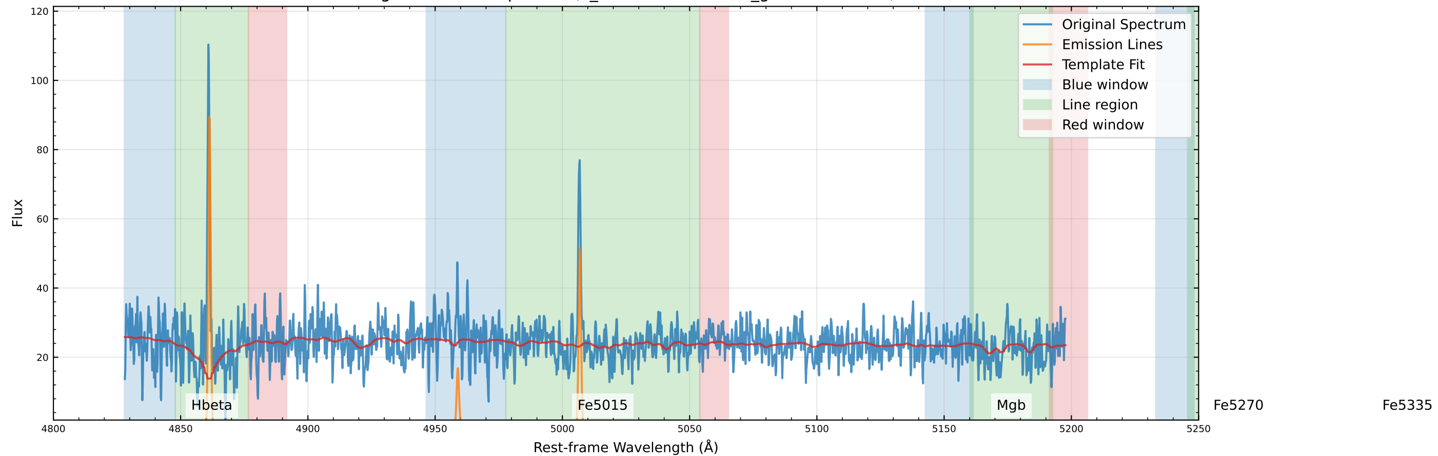
Original Data Comparison (v_star=-35.2 km/s, v_gas=-19.3 km/s)
