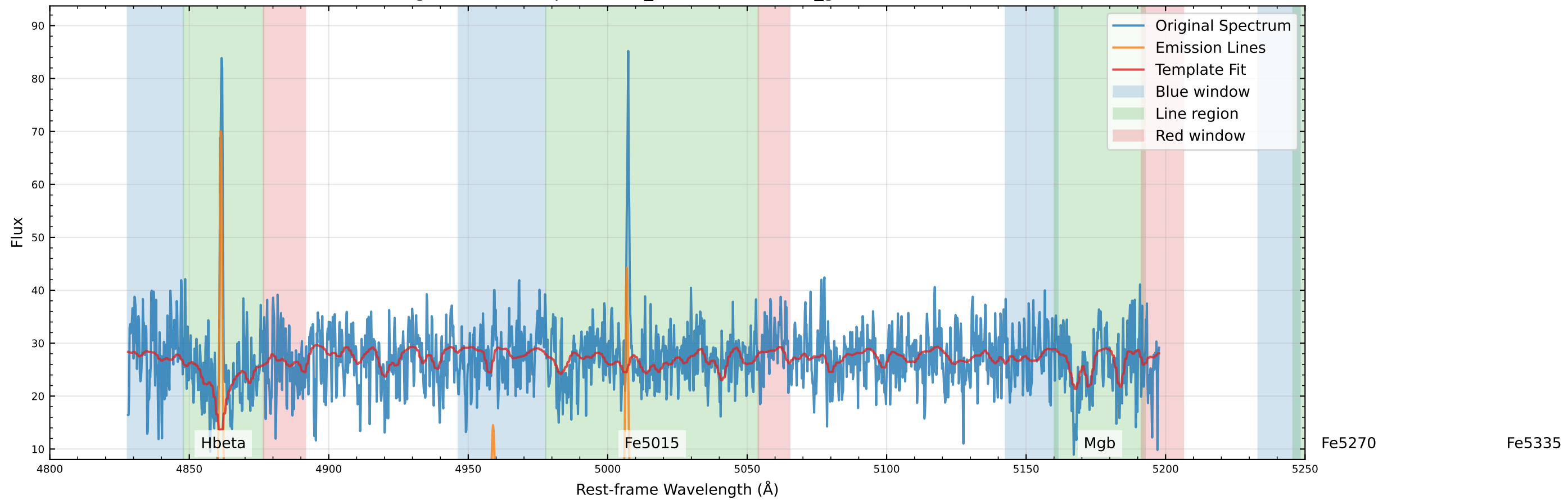
Original Data Comparison (v_star=14.2 km/s, v_gas=17.6 km/s)
