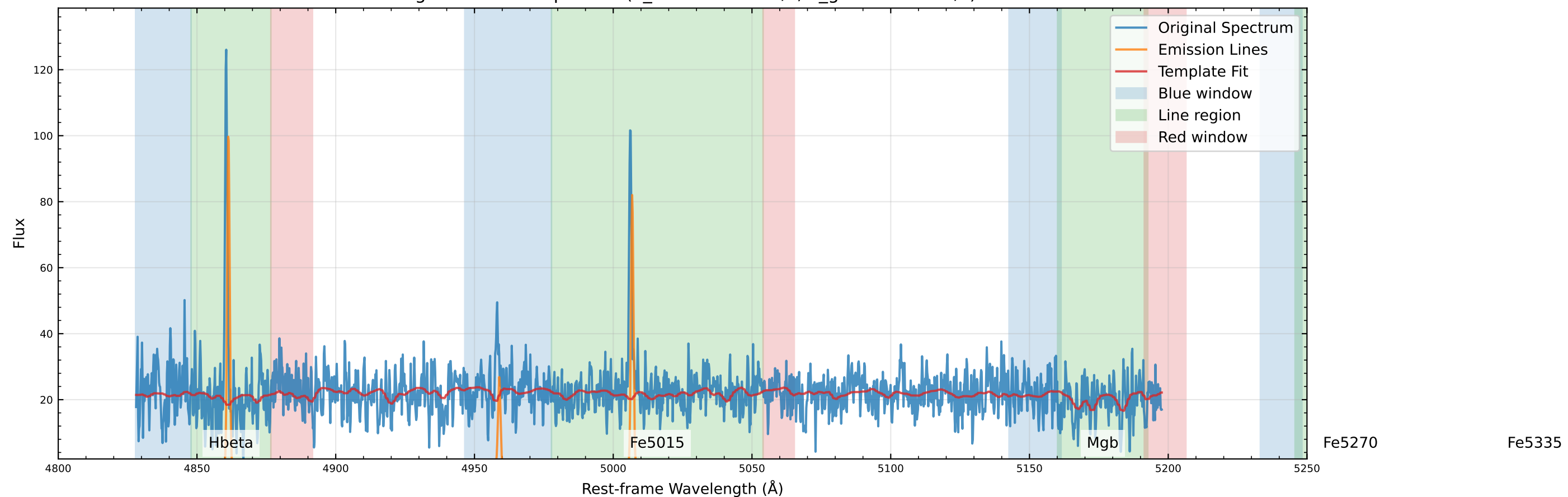
Original Data Comparison (v_star=-21.2 km/s, v_gas=-46.0 km/s)
