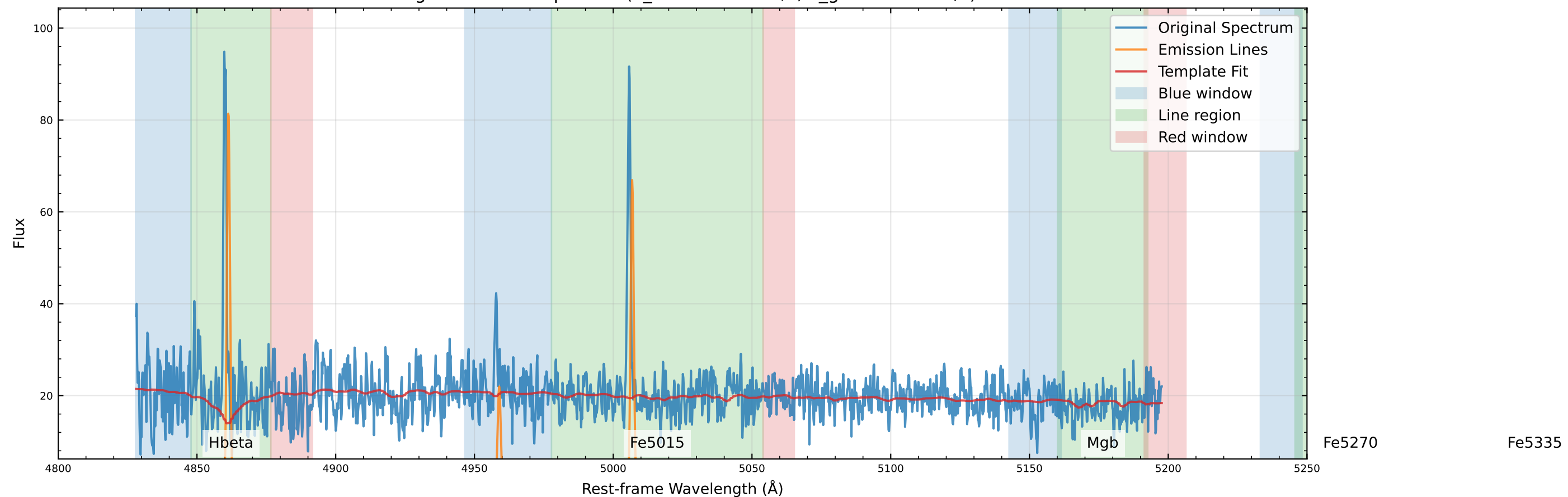
Original Data Comparison ( v_{\text{star}}=-68.8 km/s, v_{\text{gas}}=-73.1 km/s)
