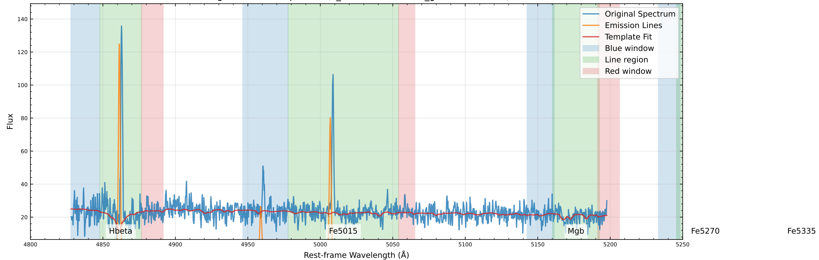
Original Data Comparison (v_star=59.4 km/s, v_gas=102.0 km/s)
