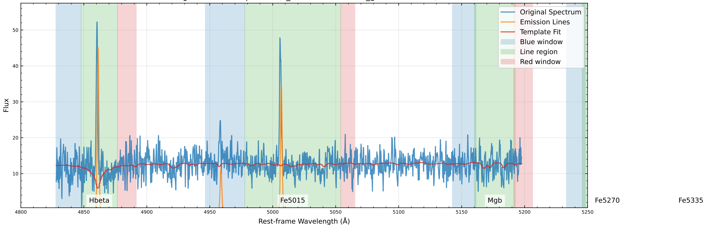
Original Data Comparison (v_star=-59.0 km/s, v_gas=-53.0 km/s)
