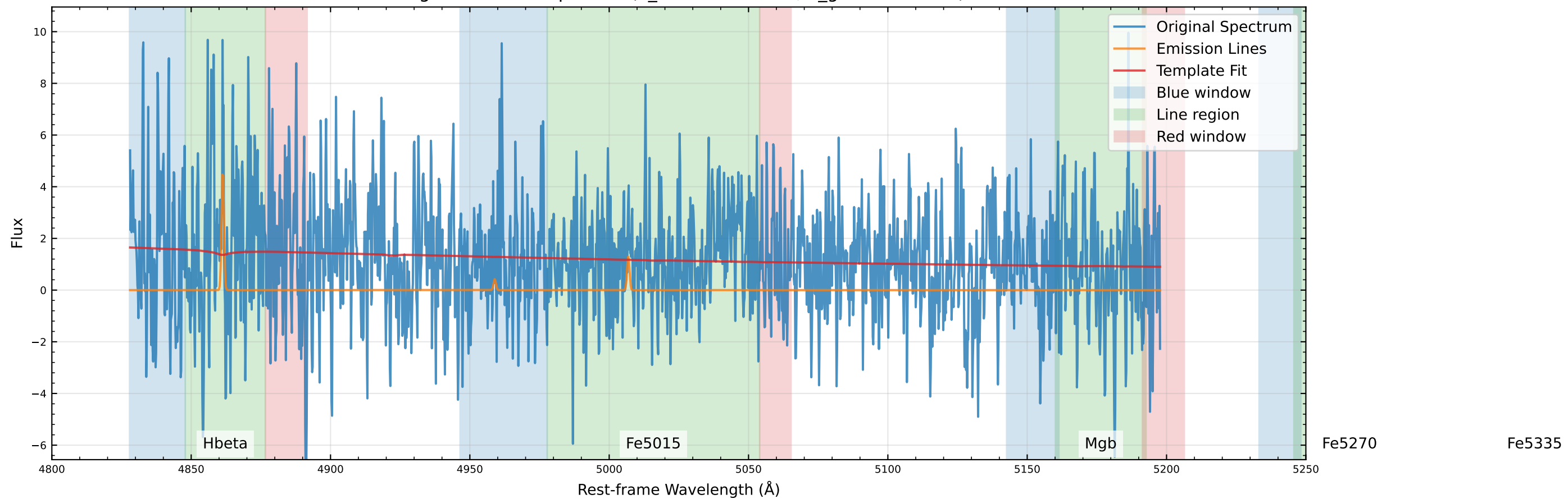
Original Data Comparison (v_star=29.4 km/s, v_gas=-2.2 km/s)
