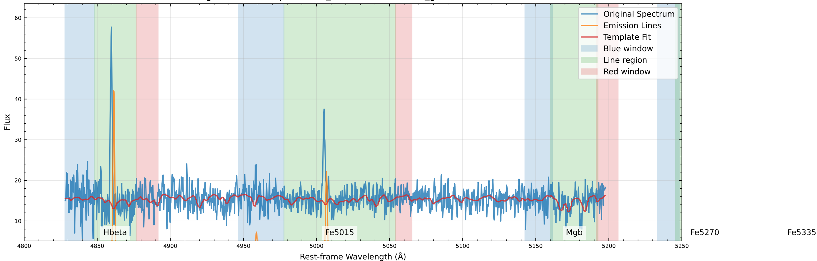
Original Data Comparison (v_star=-105.9 km/s, v_gas=-107.4 km/s)
