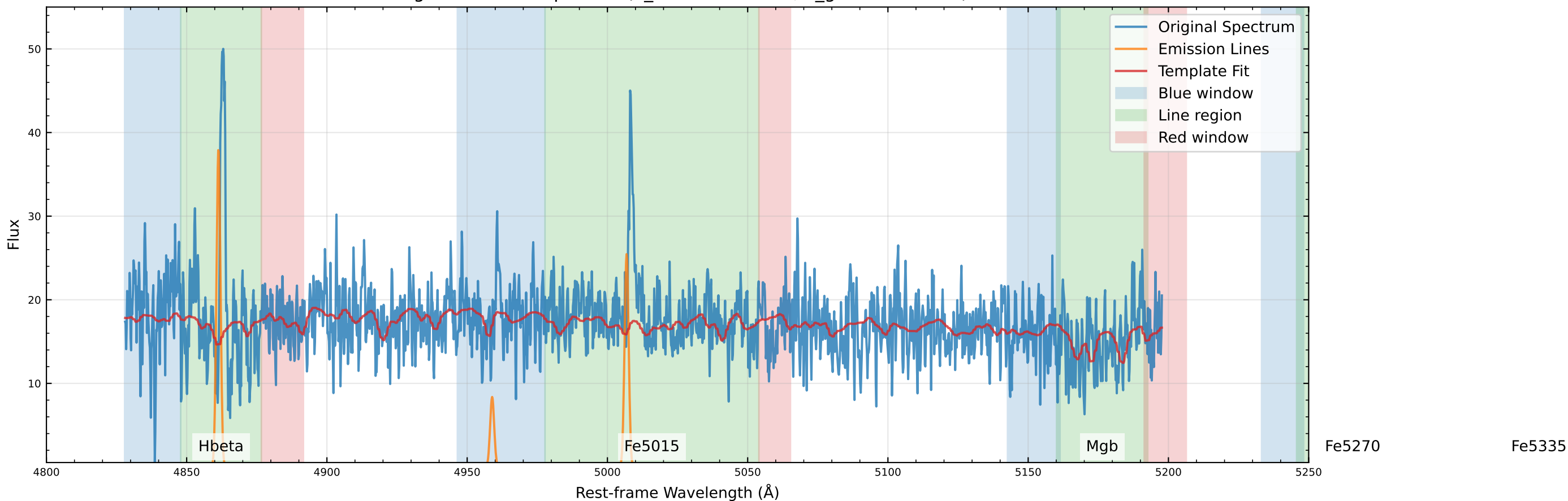
Original Data Comparison (v_star=13.8 km/s, v_gas=95.4 km/s)
