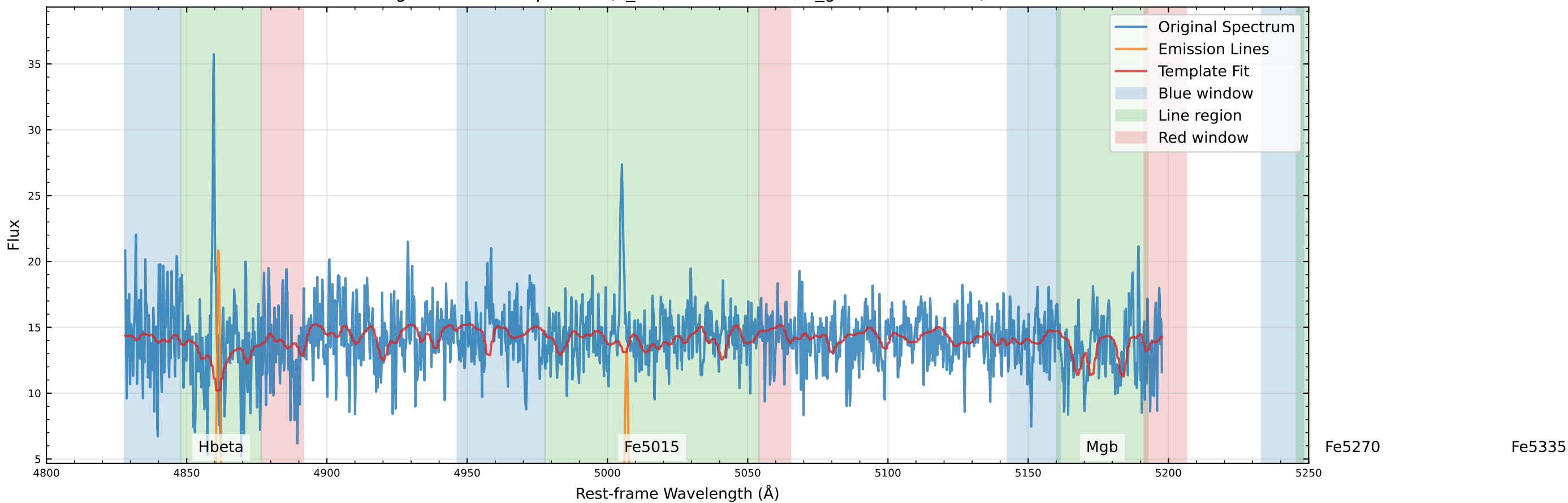
Original Data Comparison (v_star=-118.6 km/s, v_gas=-105.5 km/s)
