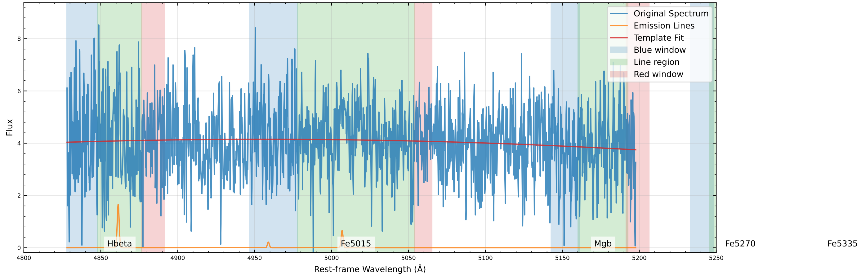
Original Data Comparison (v_star=-219.3 km/s, v_gas=-164.1 km/s)
