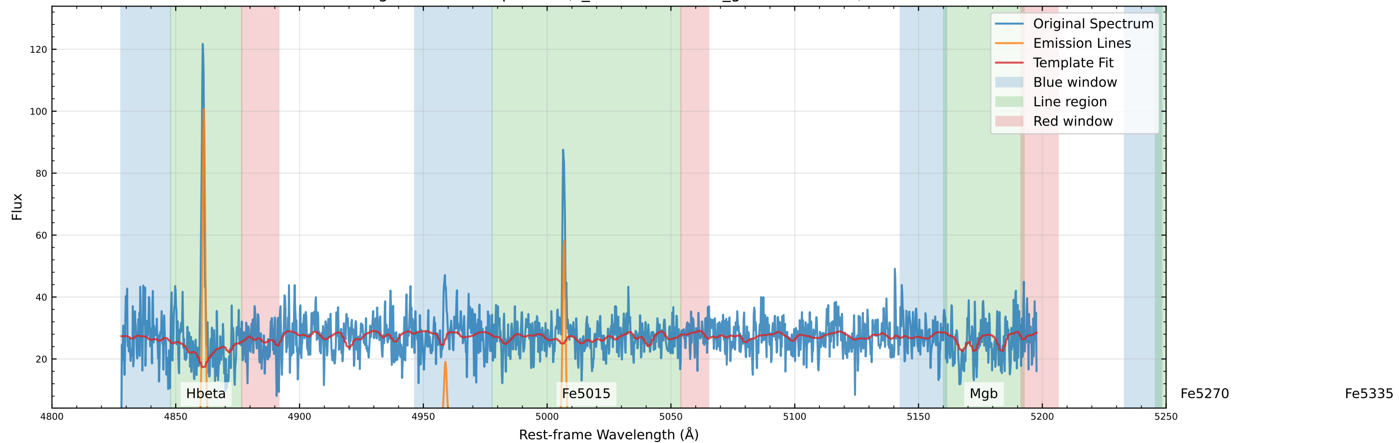
Original Data Comparison (v_star=2.8 km/s, v_gas=-19.0 km/s)
