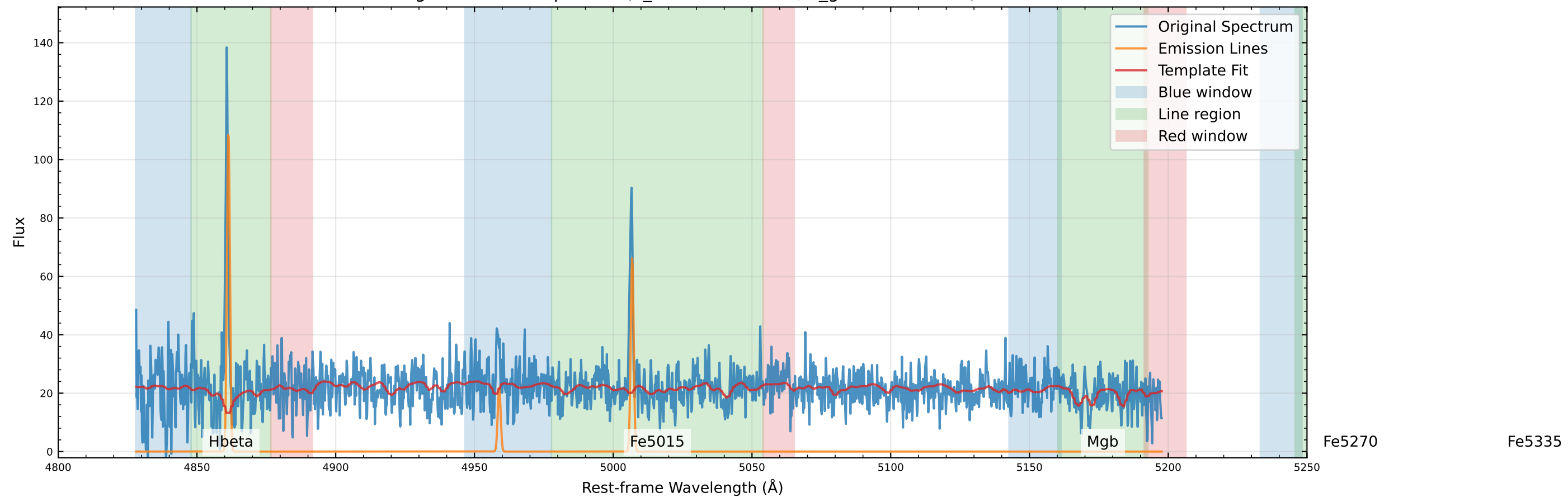
Original Data Comparison (v_star=-22.7 km/s, v_gas=-32.5 km/s)
