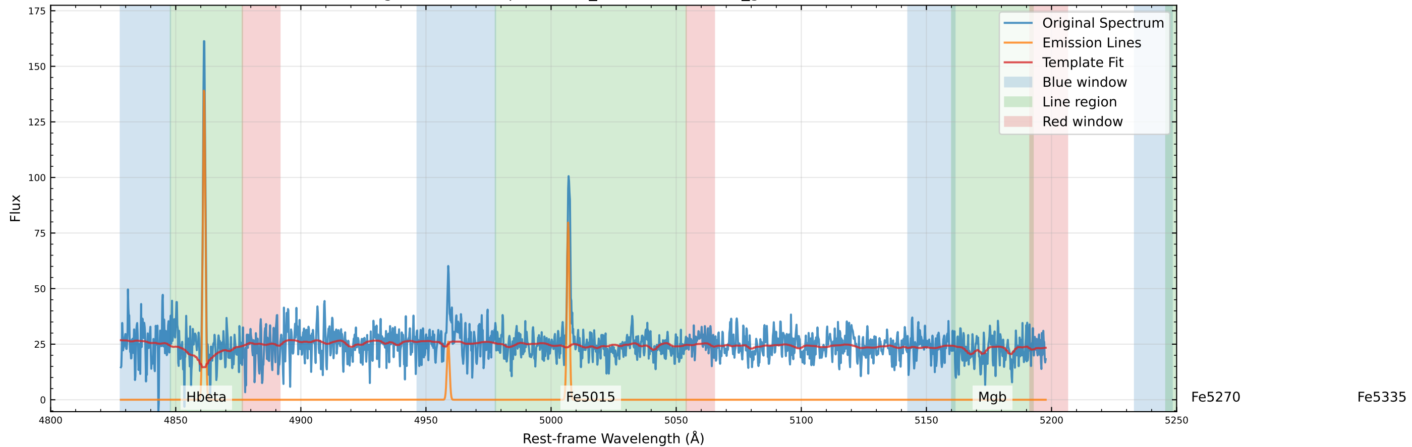
Original Data Comparison (v_star=20.5 km/s, v_gas=5.6 km/s)
