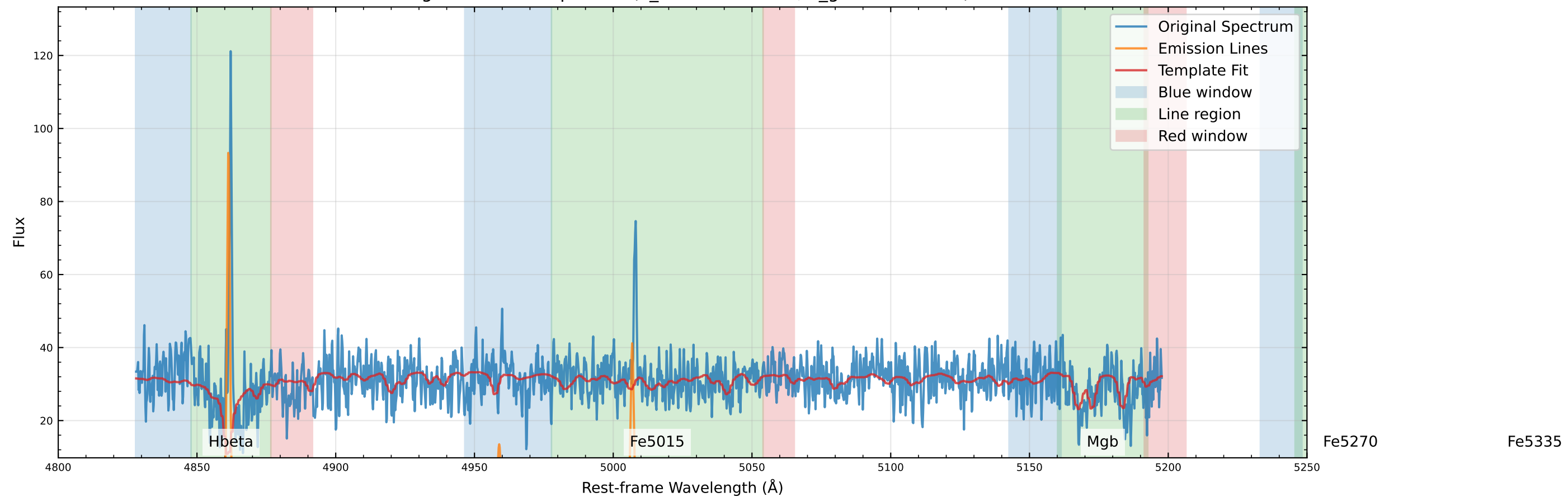
Original Data Comparison (v_star=59.6 km/s, v_gas=52.4 km/s)
