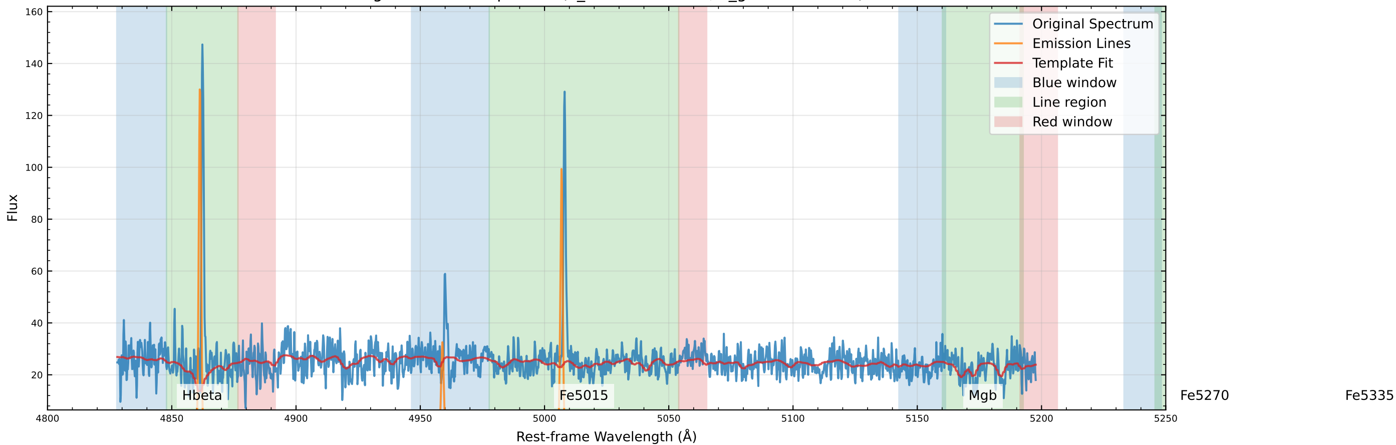
Original Data Comparison (v_star=61.5 km/s, v_gas=69.8 km/s)
