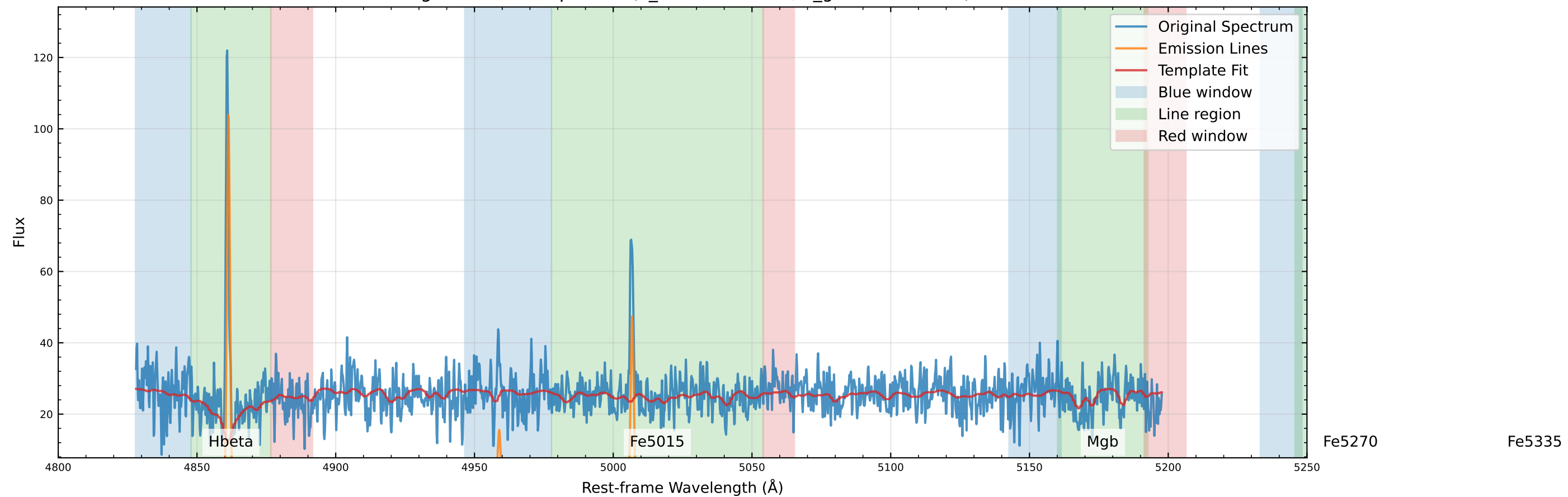
Original Data Comparison (v_star=-9.4 km/s, v_gas=-24.0 km/s)
