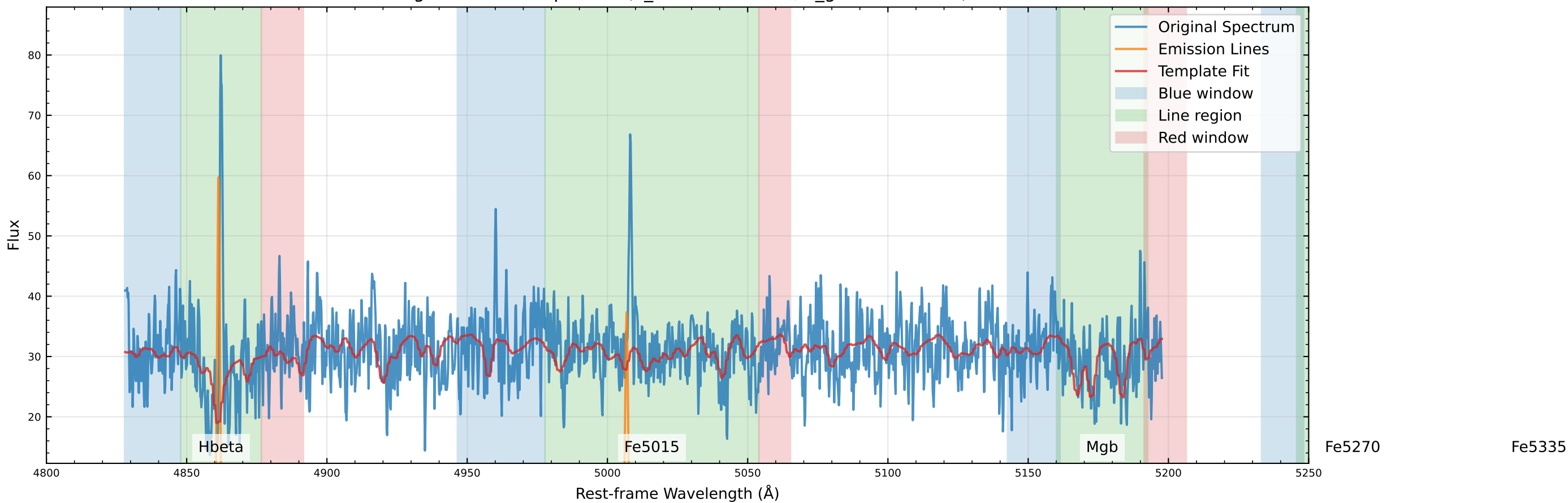
Original Data Comparison (v_star=74.5 km/s, v_gas=65.2 km/s)
