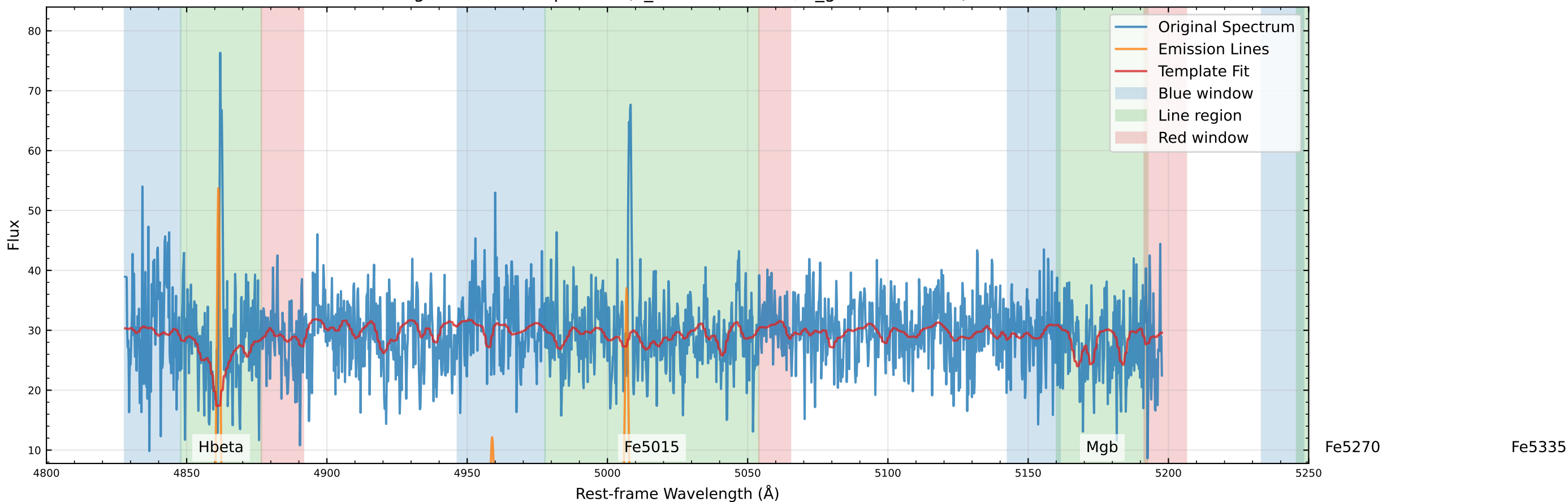
Original Data Comparison (v_star=63.9 km/s, v_gas=62.4 km/s)
