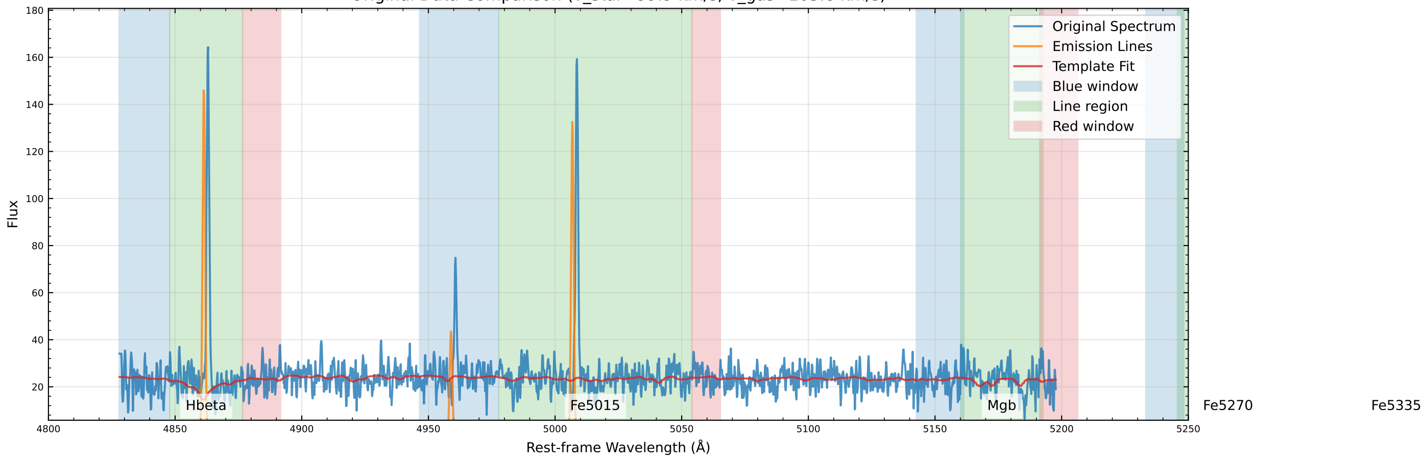
Original Data Comparison (v_star=99.9 km/s, v_gas=103.8 km/s)
