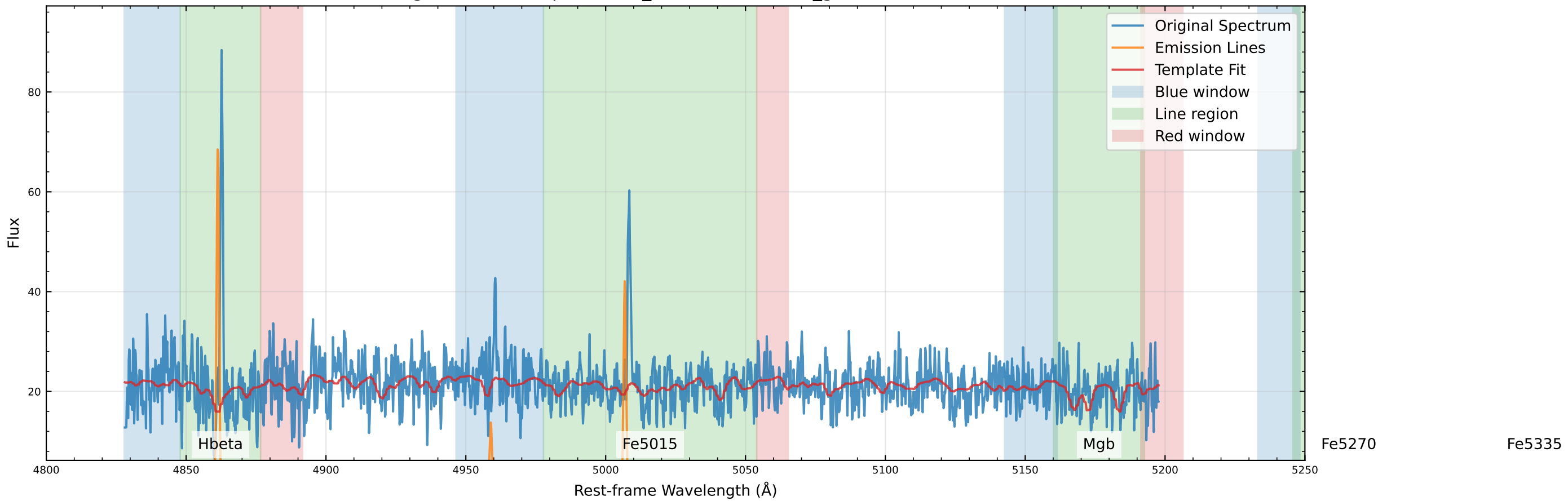
Original Data Comparison (v_star=81.6 km/s, v_gas=85.7 km/s)
