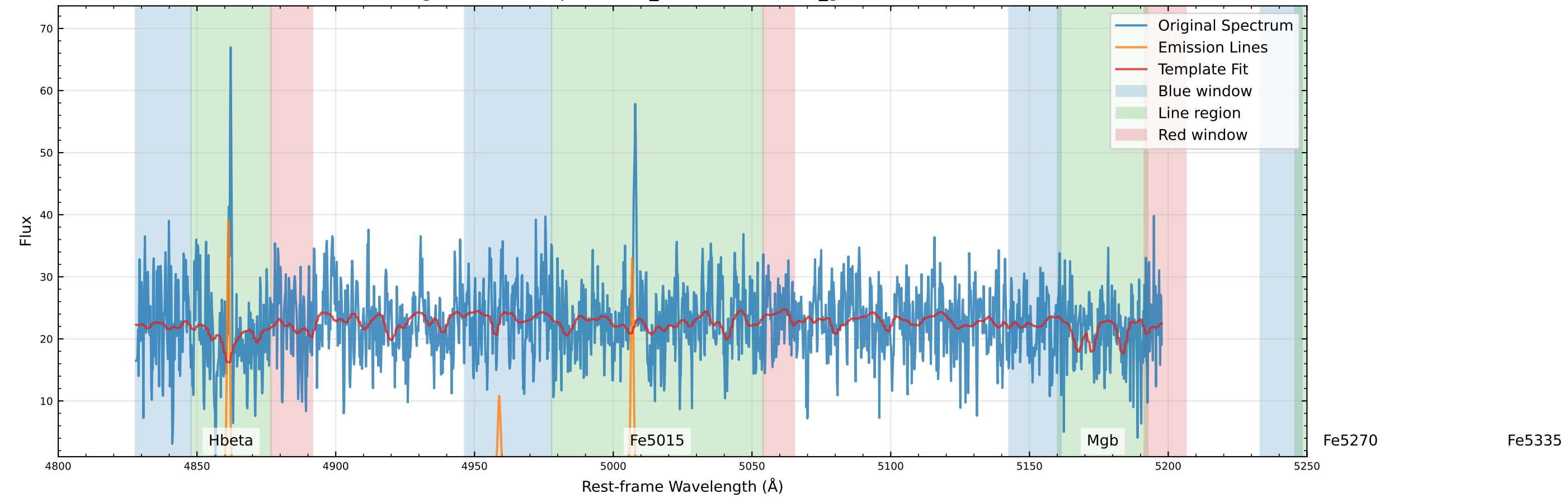
Original Data Comparison (v_star=66.3 km/s, v_gas=50.2 km/s)
