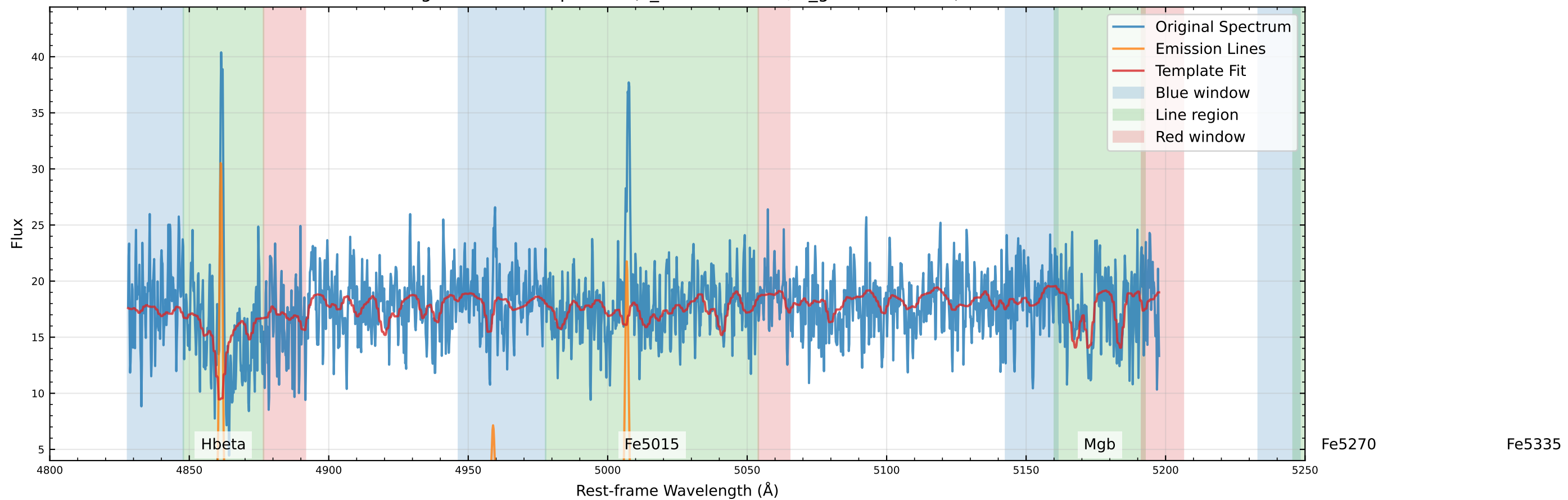
Original Data Comparison (v_star=7.8 km/s, v_gas=22.6 km/s)
