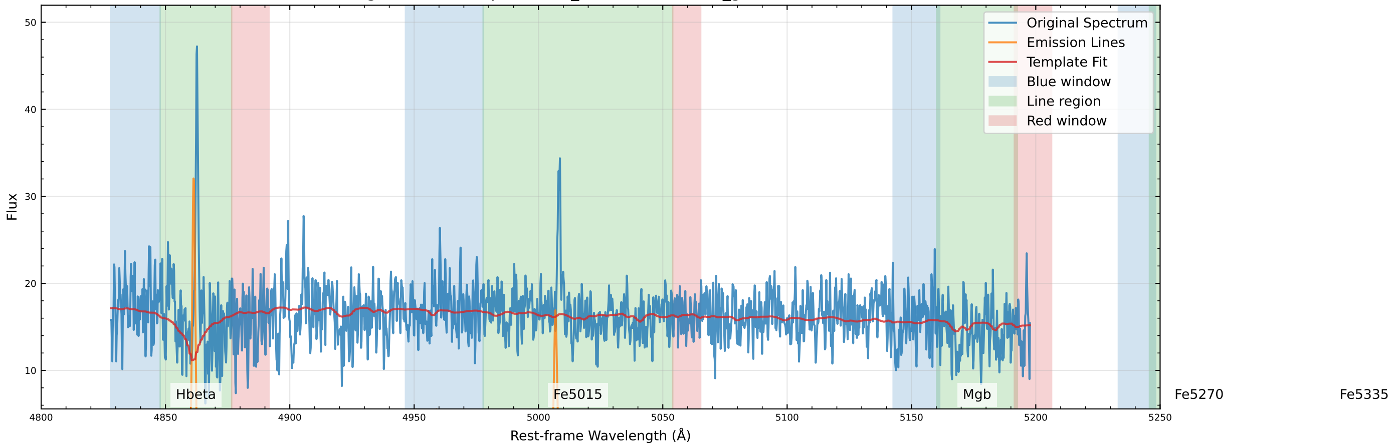
Original Data Comparison (v_star=81.3 km/s, v_gas=81.2 km/s)
