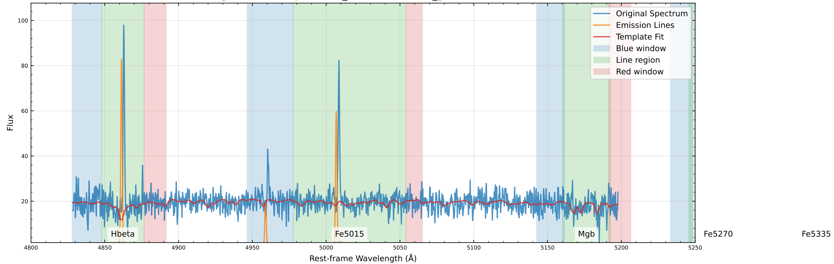
Original Data Comparison (v_star=90.6 km/s, v_gas=100.7 km/s)
