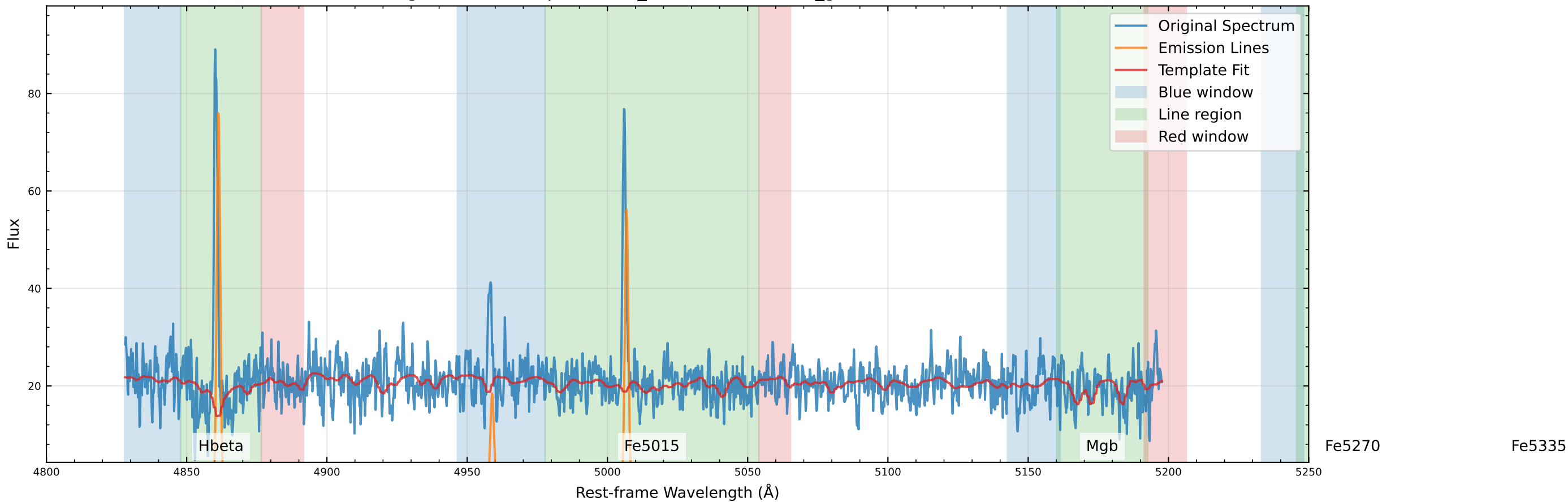
Original Data Comparison (v_star=-48.5 km/s, v_gas=-55.1 km/s)
