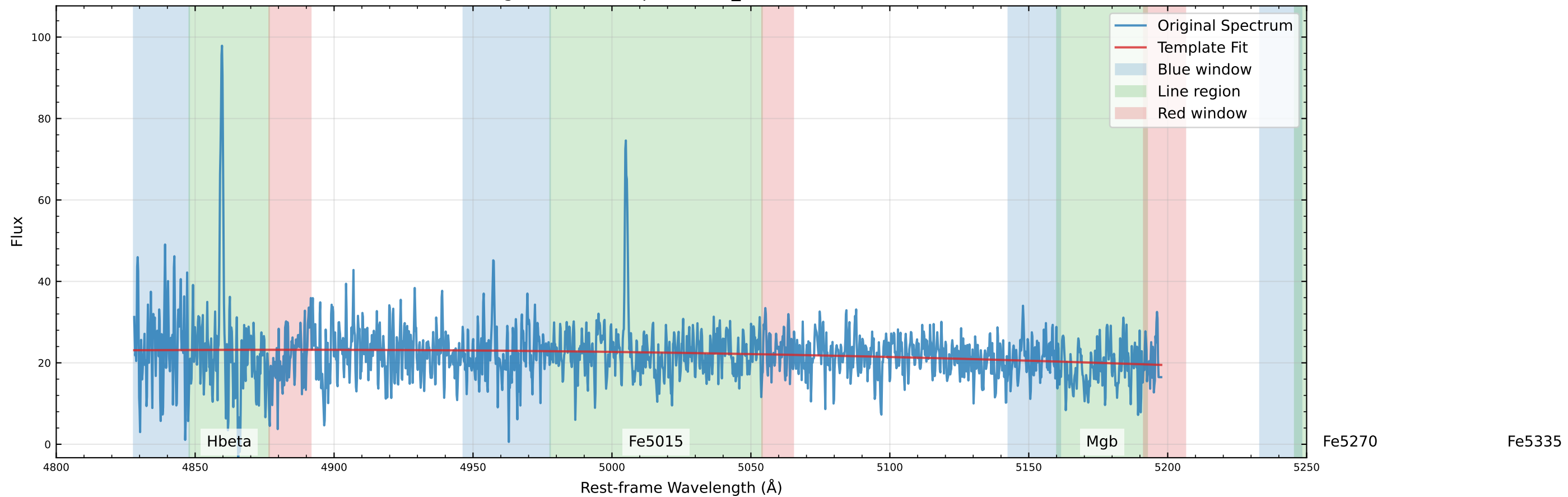
Original Data Comparison (v_star=28.9 km/s)
