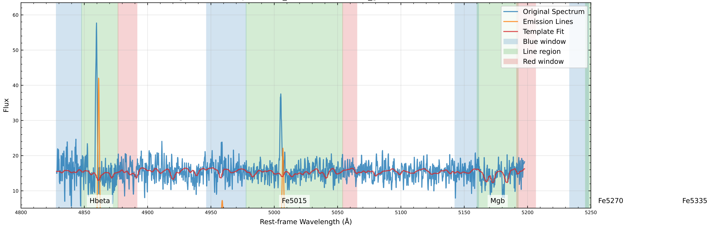
Original Data Comparison (v_star=-105.9 km/s, v_gas=-107.4 km/s)
