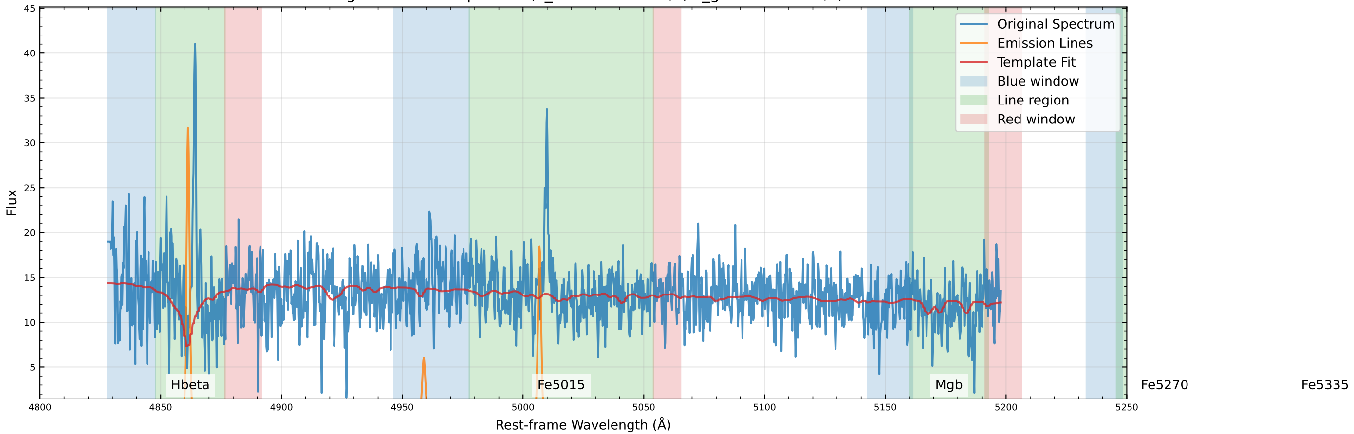
Original Data Comparison (v_star=166.5 km/s, v_gas=170.1 km/s)
