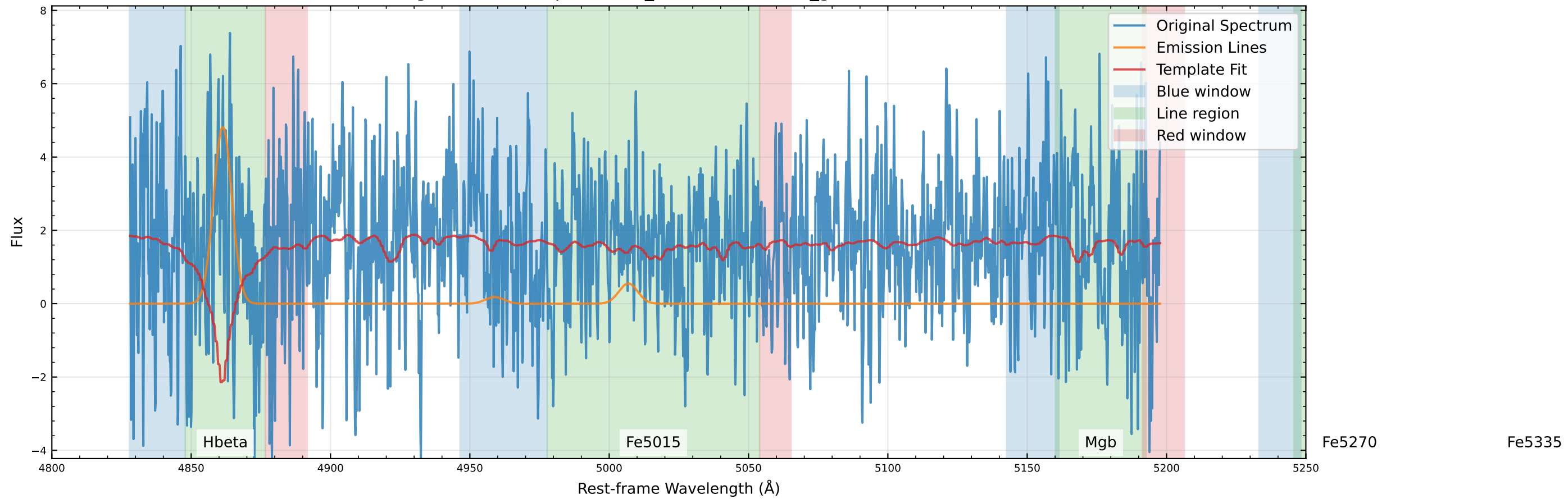
Original Data Comparison (v_star=-3.8 km/s, v_gas=-24.1 km/s)
