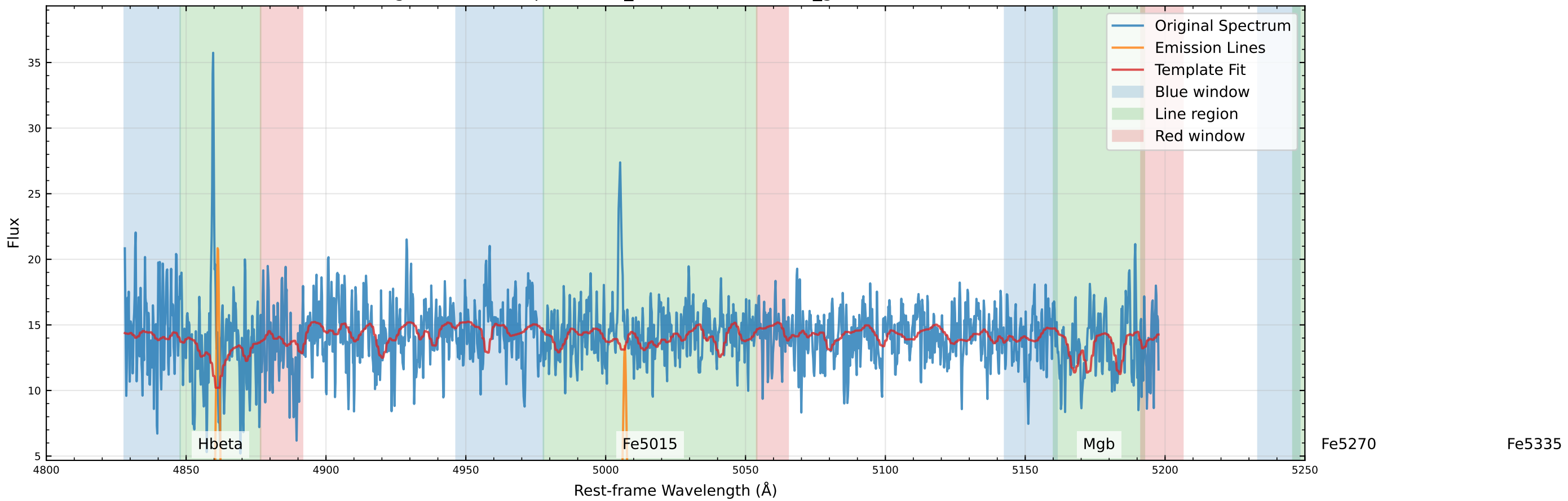
Original Data Comparison (v_star=-118.6 km/s, v_gas=-105.5 km/s)
