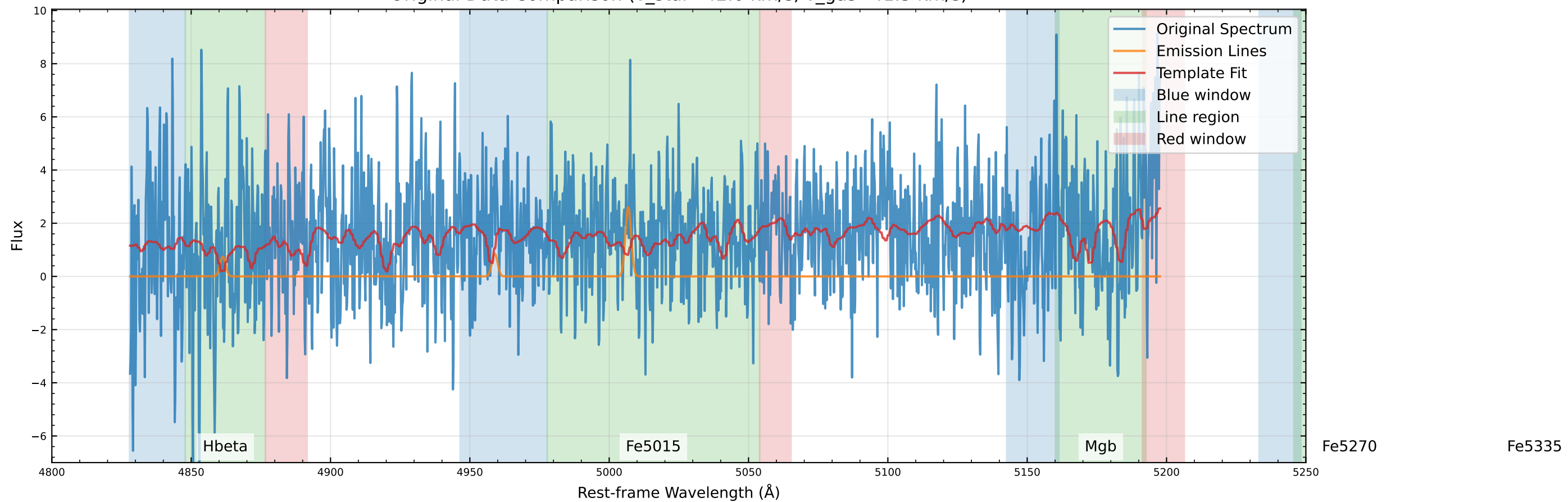
Original Data Comparison (v_star=42.0 km/s, v_gas=41.3 km/s)
