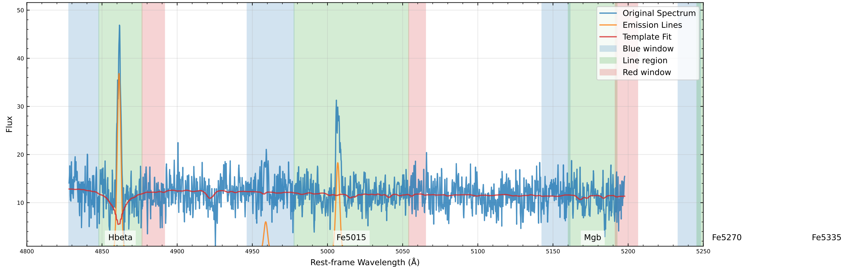
Original Data Comparison (v_star=108.6 km/s, v_gas=7.6 km/s)
