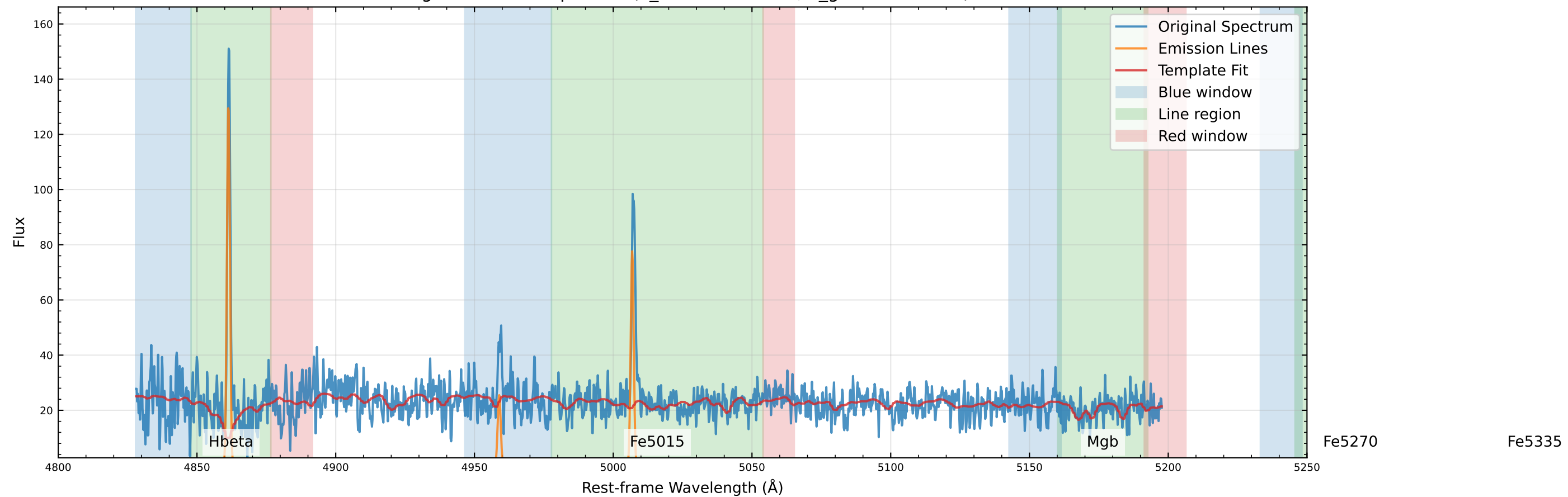
Original Data Comparison (v_star=25.8 km/s, v_gas=14.4 km/s)
