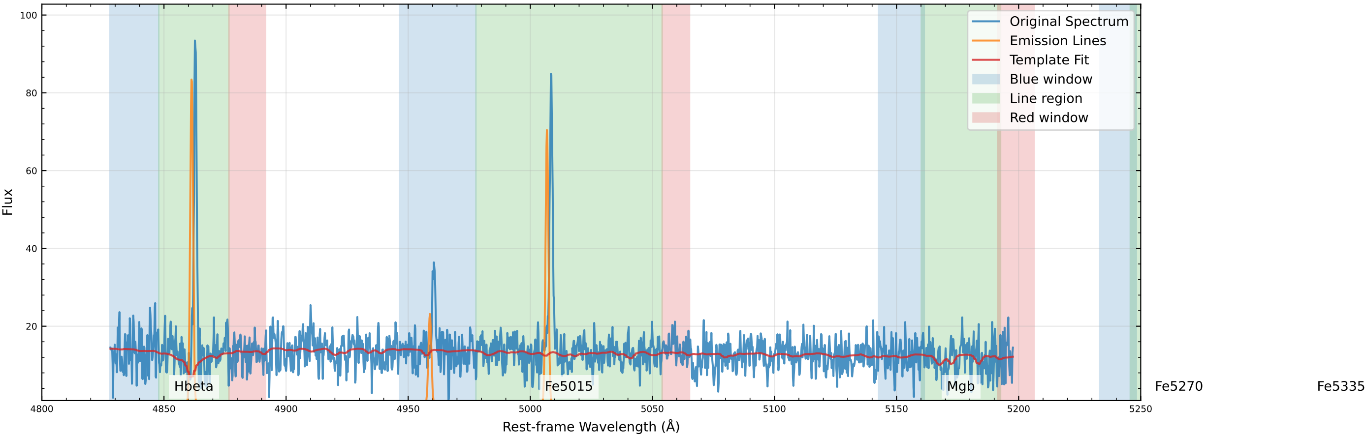
Original Data Comparison (v_star=85.7 km/s, v_gas=96.6 km/s)
