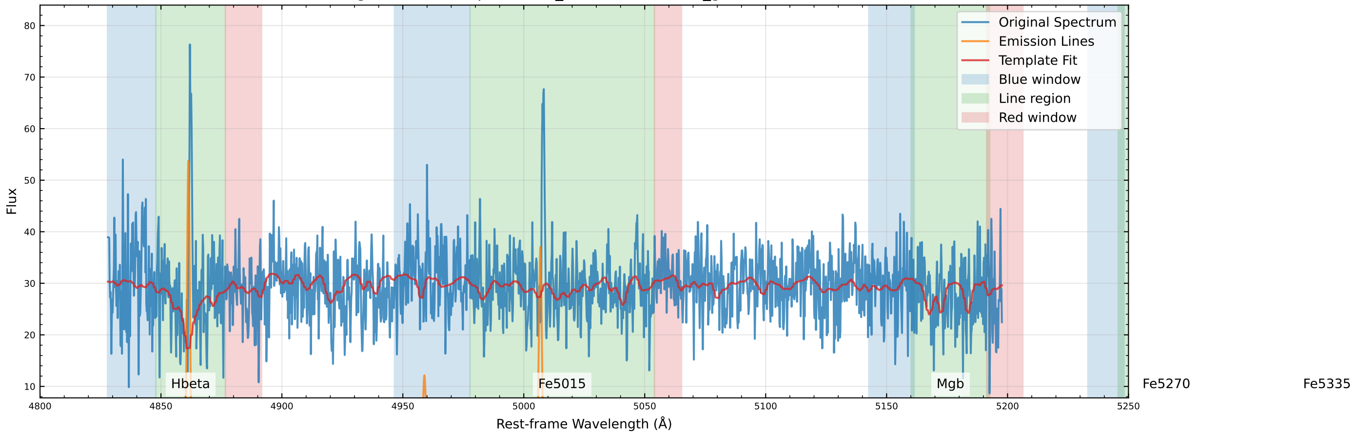
Original Data Comparison (v_star=63.9 km/s, v_gas=62.4 km/s)
