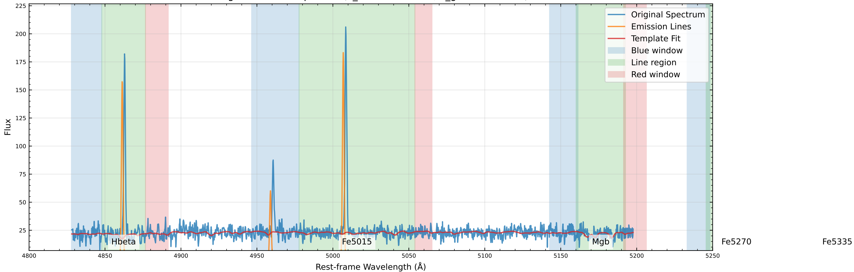
Original Data Comparison (v_star=86.0 km/s, v_gas=99.4 km/s)
