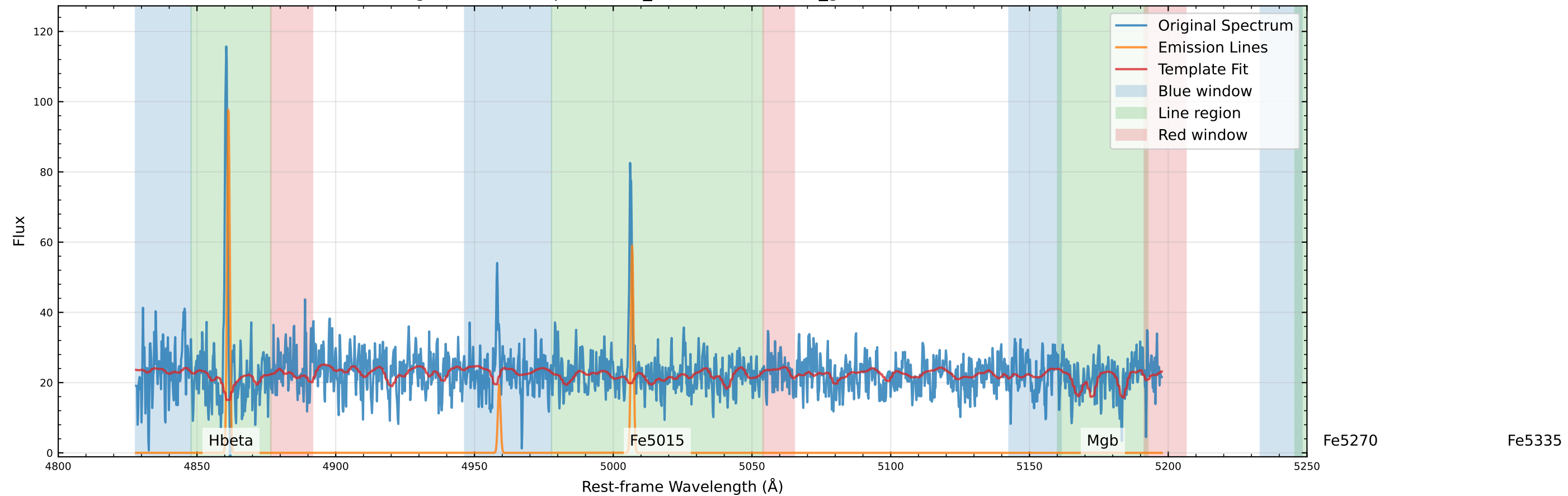
Original Data Comparison (v_star=-33.7 km/s, v_gas=-46.6 km/s)
