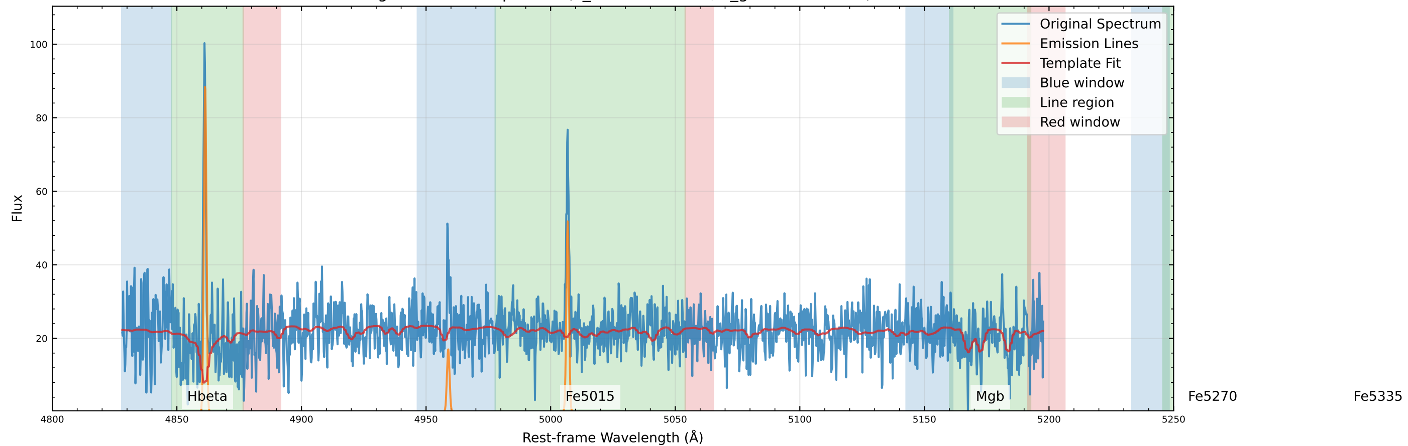
Original Data Comparison (v_star=-2.9 km/s, v_gas=-11.5 km/s)
