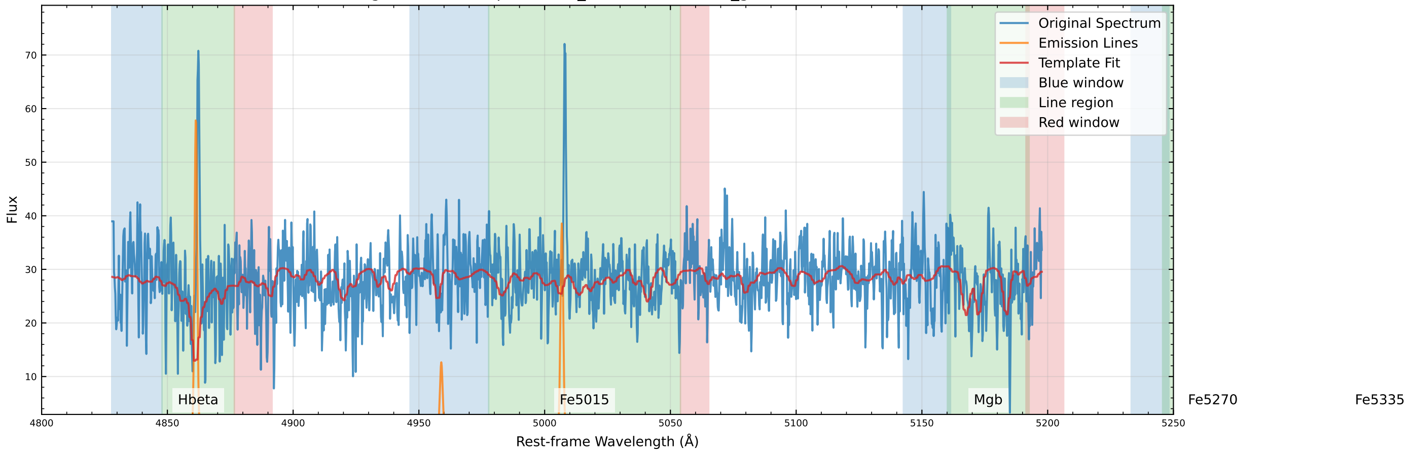
Original Data Comparison (v_star=65.0 km/s, v_gas=65.8 km/s)
