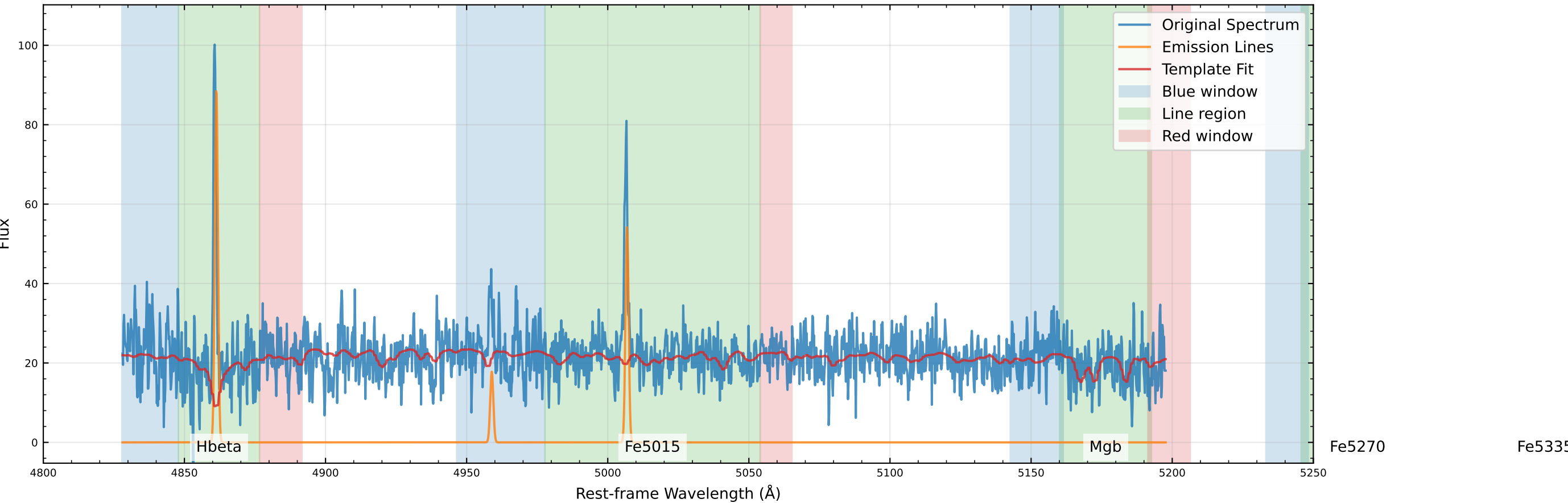
Original Data Comparison (v_star=-56.4 km/s, v_gas=-33.1 km/s)
