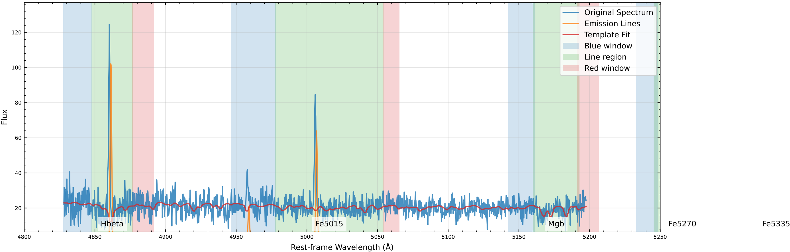
Original Data Comparison (v_star=-79.4 km/s, v_gas=-66.9 km/s)
