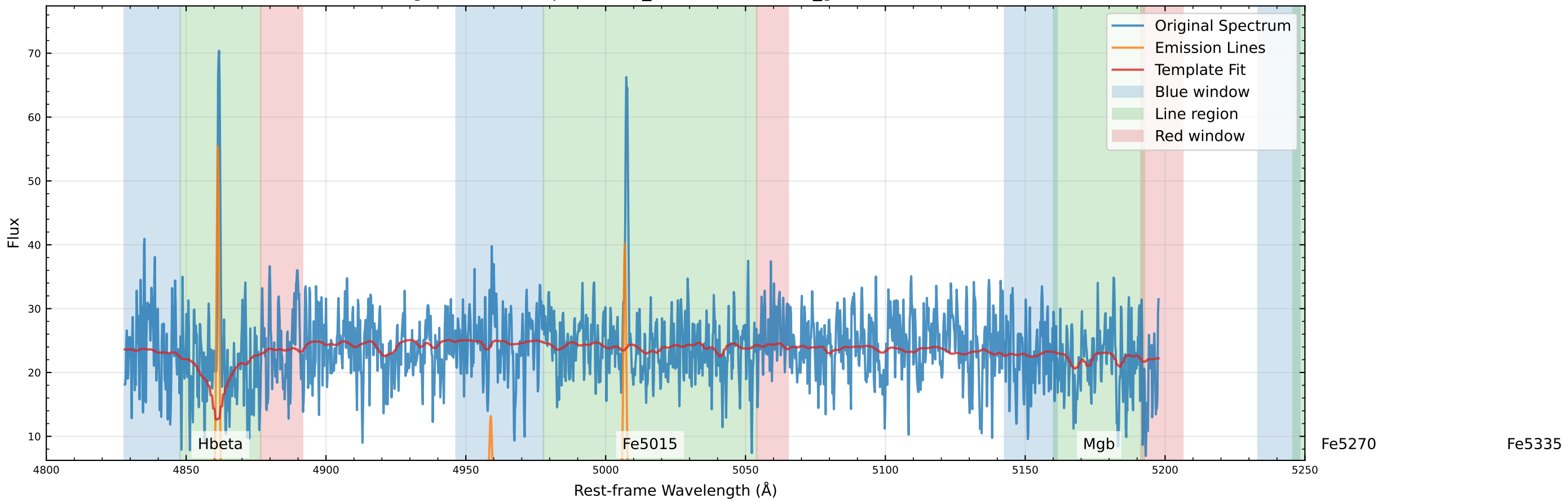
Original Data Comparison (v_star=34.1 km/s, v_gas=30.4 km/s)
