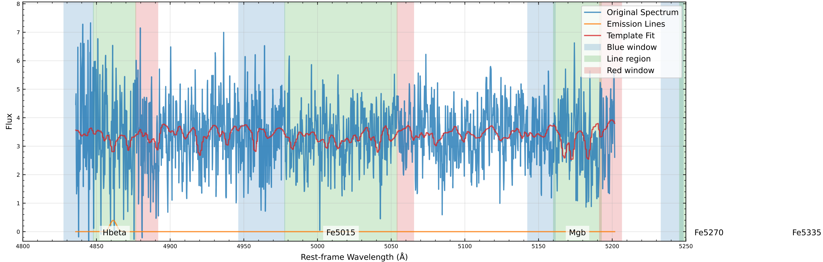
Original Data Comparison (v_star=194.6 km/s, v_gas=230.3 km/s)
