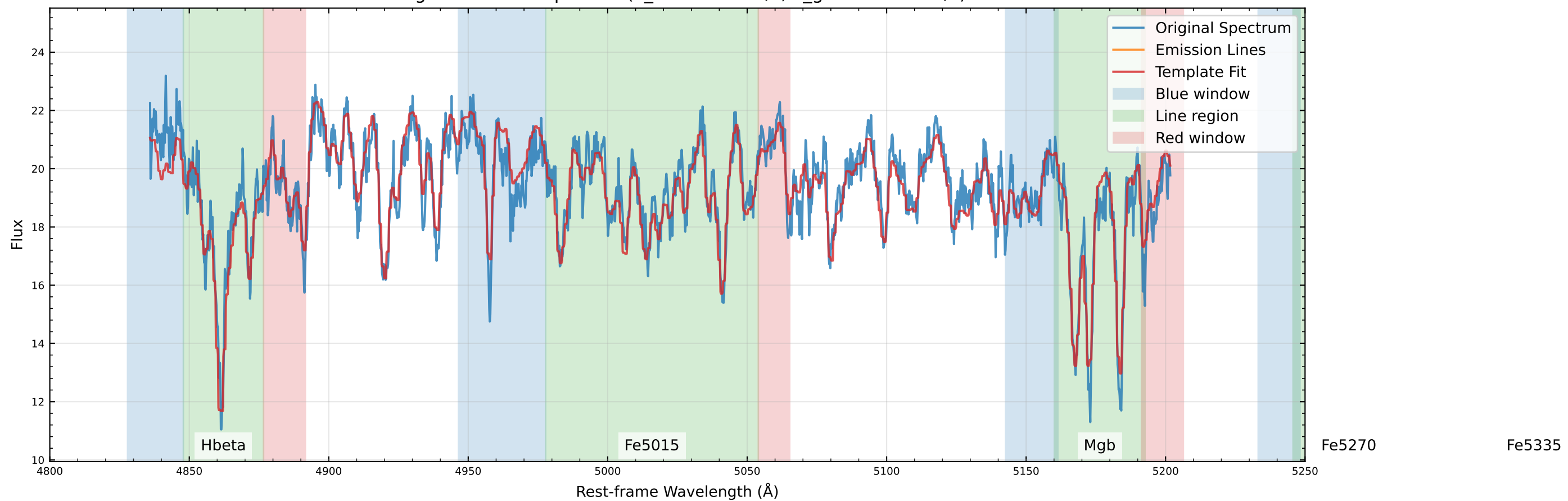
Original Data Comparison (v_star=6.8 km/s, v_gas=233.3 km/s)
