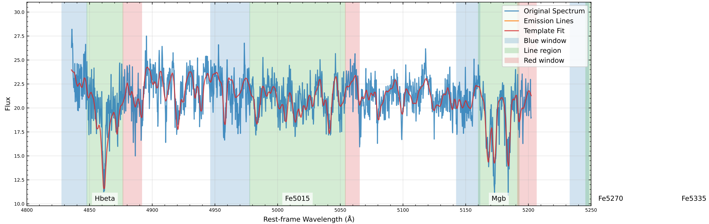
Original Data Comparison (v_star=21.7 km/s, v_gas=-0.5 km/s)
