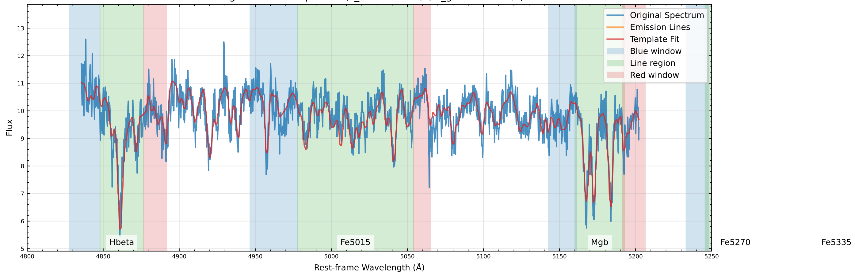
Original Data Comparison (v_star=1.1 km/s, v_gas=20.9 km/s)
