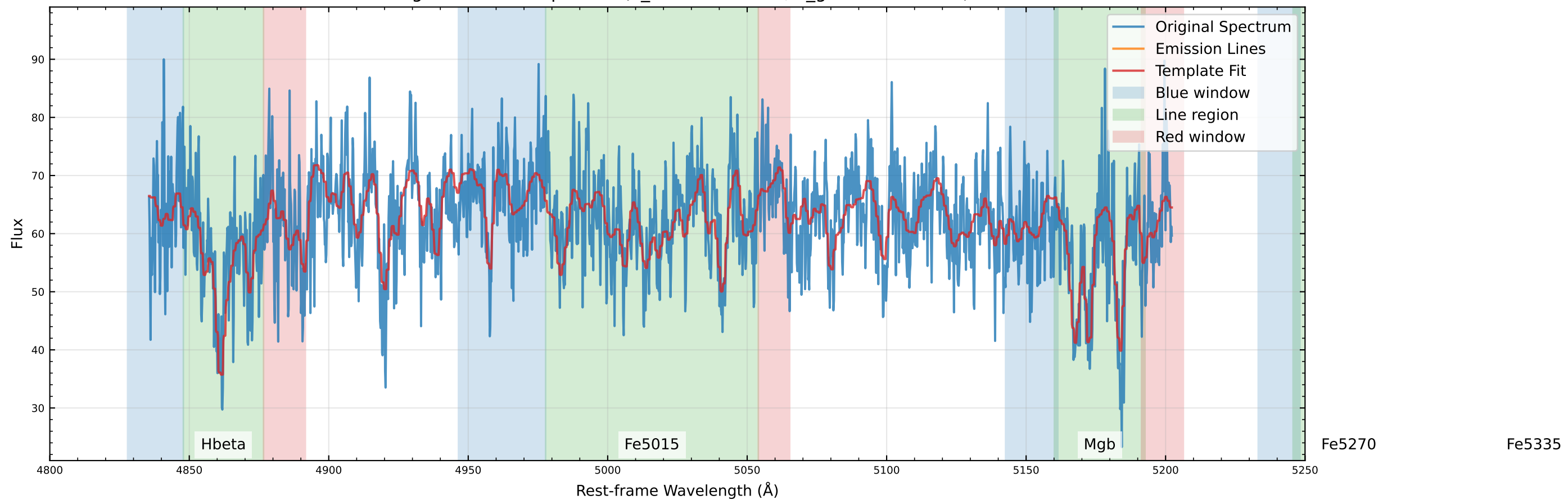
Original Data Comparison (v_star=-0.6 km/s, v_gas=128.4 km/s)
